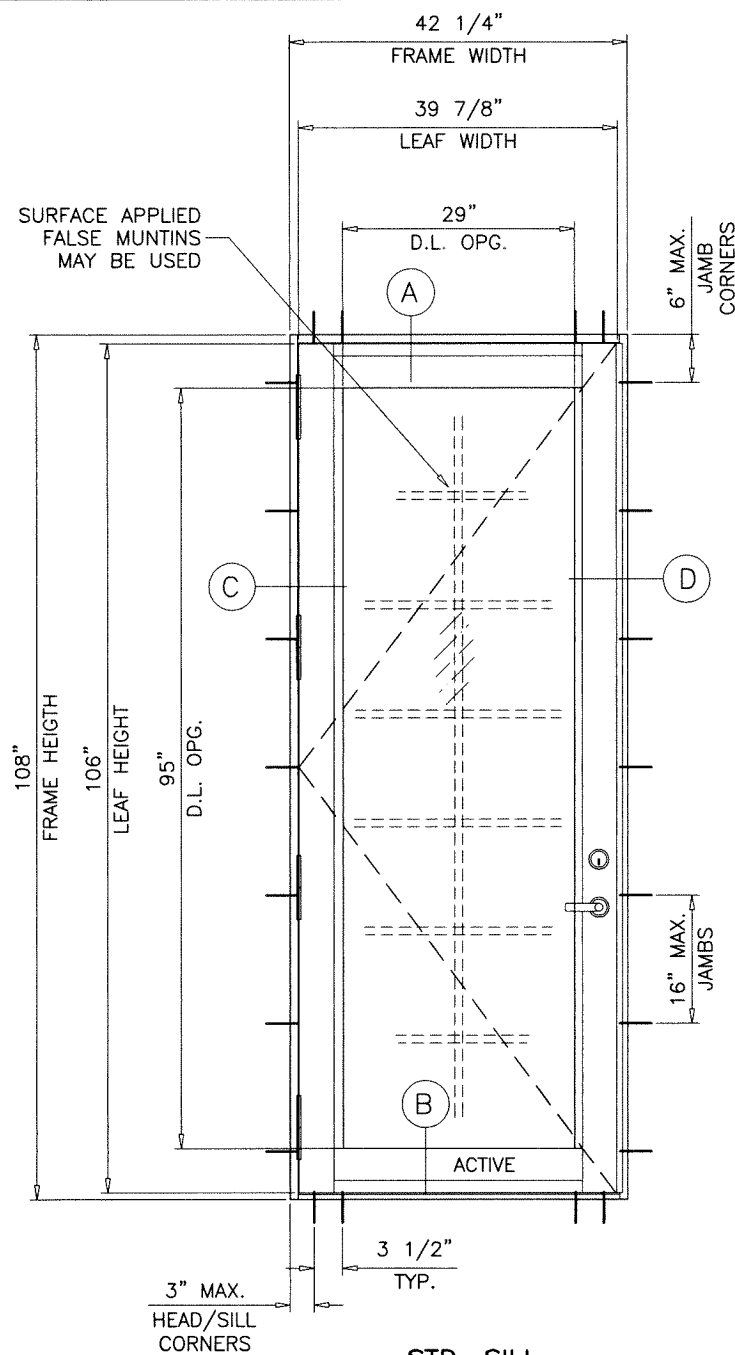
STD. SILL TYPICAL ELEVATION ( X )
